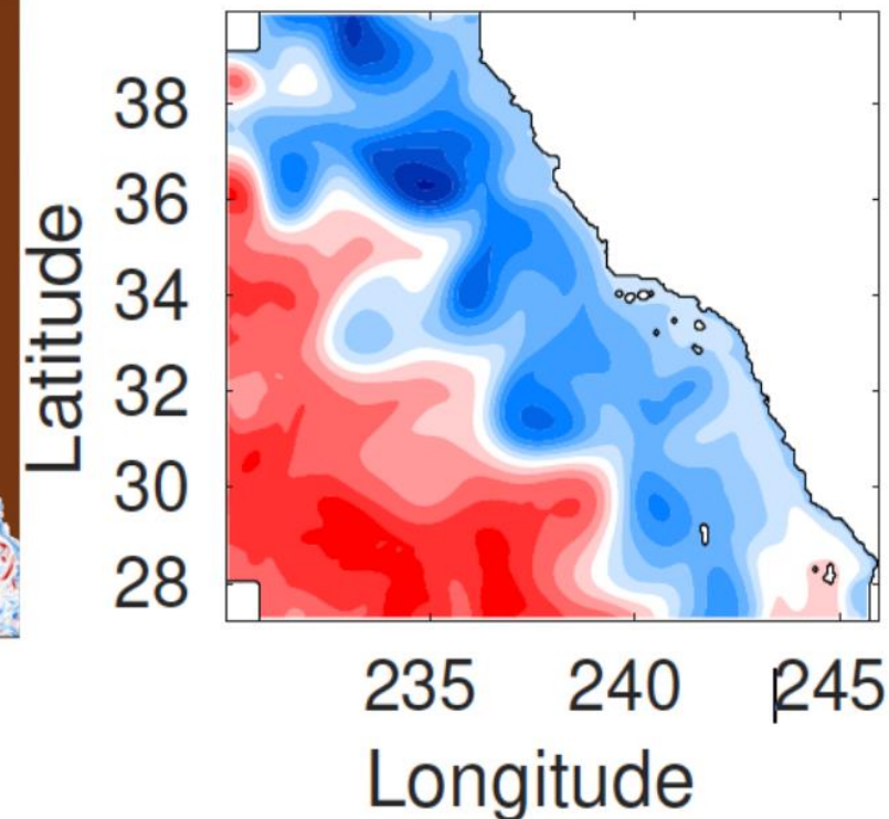
SIO and JPL: 4-D Var using MITgcm
